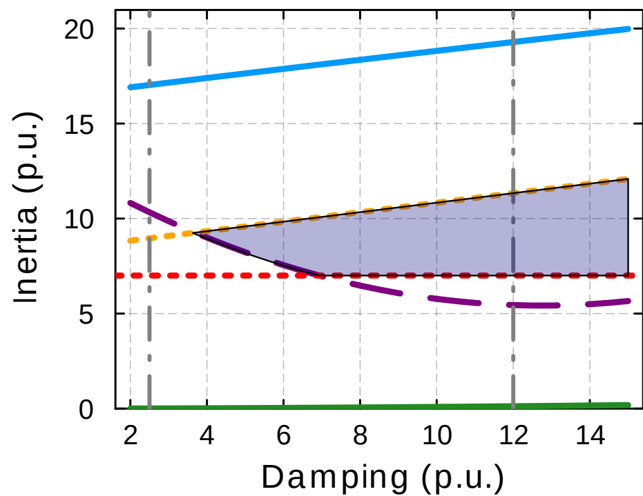
(c) Droop = 0.029
